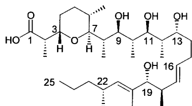
Figure 1. Structure of zincphorin.
